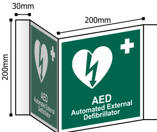
200 x 200 RPVC 4465
